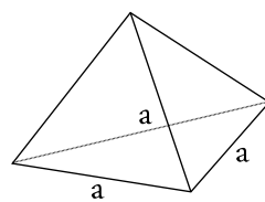
tetraeder a^3 \times \sqrt{2} / 12
