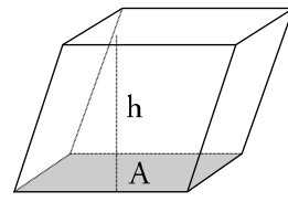
parallelepiped A \times h
