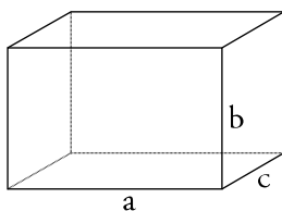
rätblock a \times b \times c
