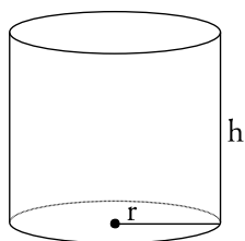
cylinder \pi \times r^2 \times h
